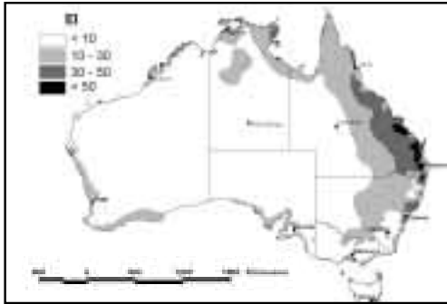
Figure 3. Potential distribution of parthenium weed. (Data is splined from a CLIMEX climate prediction. EI=Ecoclimatic Index: EI < 10 potential for permanent population low, EI > 50 potential very high).
